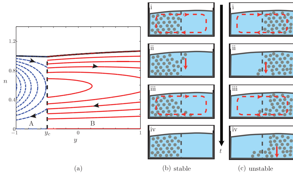
FIG. 4. (a) The streamlines of the particle-laden flow are computed for \lambda = \epsilon = 0.29 . The cross-section is divided into two regions: region A (dotted lines, \psi = -C_A \times 10^{-5} , C_A = 0, 0.5, \dots, 3.5 ) denotes the particle-rich region, while region B (solid lines, \psi = -C_B \times 10^{-3} , C_B = 0, 0.5, \dots, 2.5 ) consists only of the clear fluid. The arrows indicate the direction of the clockwise secondary flow and the free surface and channel bottom correspond to \psi = 0 . Two equilibrium configurations are depicted in (b) and (c), along with their time evolution, from top (i) to bottom (iv), as a result of perturbation by the secondary flow. The configuration in (b) is stable, while that in (c) is unstable.
