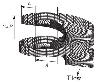
FIG. 1. A helical channel of rectangular cross section of width 2a . The spiral radius is A , while the vertical spacing between each turn is the pitch 2\pi P .
