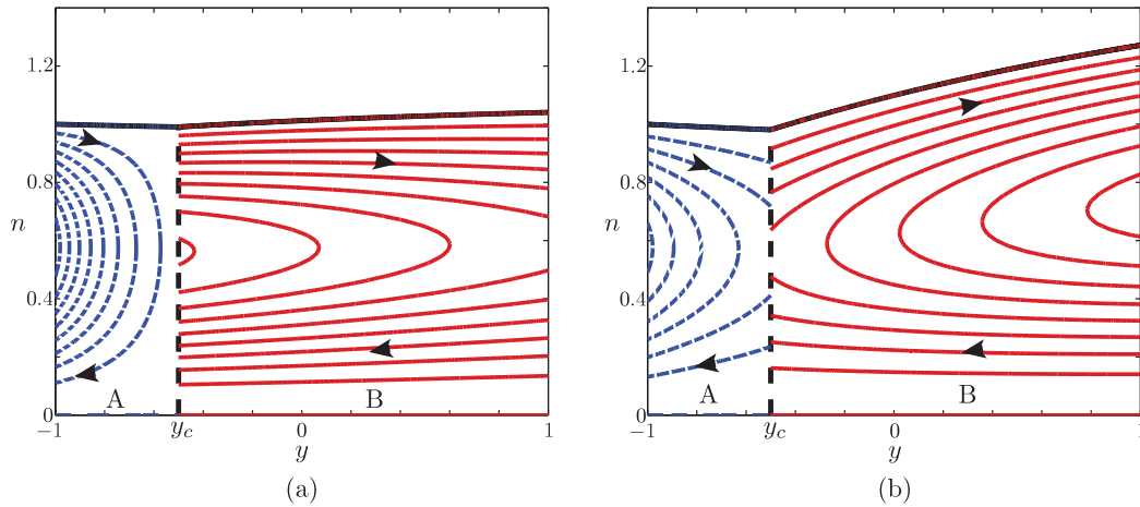
FIG. 6. The plots of streamlines for (a) \lambda = \epsilon = 0.25 , \psi = -C_A \times 10^{-6} , C_A = 0, 1, \dots, 8 (dotted lines), \psi = -C_B \times 10^{-3} , C_B = 0, 0.2, \dots, 1.6 (solid lines), and (b) \lambda = \epsilon = 0.4 , \psi = -C_A \times 10^{-4} , C_A = 0, 0.5, \dots, 3 (dotted lines), \psi = -C_B \times 10^{-2} , C_B = 0, 0.2, \dots, 1.6 (solid lines). The arrows indicate the direction of the clockwise secondary flow and the free surface and channel bottom correspond to \psi = 0 . From the streamlines we deduce that there are two clockwise-rotating cells in the channel cross section, one in each of regions A and B. Increasing the curvature \epsilon and the inclination angle \lambda of the channel axis clearly results in an increase in fluid depth with distance from the vertical helix axis.
