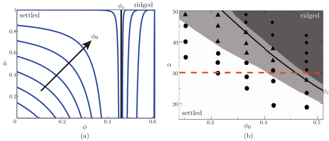
FIG. 3. (a) At the inclination angle of \alpha = 30^\circ , the profile of \phi in \tilde{n} = n/h(y) is computed for increasing values of \phi_0(y) = \int_0^1 \phi(\tilde{n}, y) d\tilde{n} ; the critical volume fraction \phi_c (constant in \tilde{n} ) is equal to 0.461. In the spiral geometry, \alpha = 30^\circ at y = 0 corresponds to setting \lambda = 1/\sqrt{3} . (b) The experimental phase diagram from Ref. 14 shows three different regimes as a function of \alpha and \phi_0 : settled (white region, dots), transient (grey region, triangles), and ridged (darker grey, diamonds). The solid line on the phase diagram is the theoretical prediction of \phi_c which sits in the transient regime, and the dotted line highlights the angle \alpha = 30^\circ from (a). Reprinted with permission from N. Murisic et al. , Physica D 240 (20), 1661–1673 (2011). Copyright 2011 Elsevier. 14
