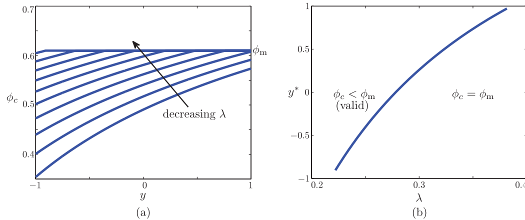
FIG. 5. (a) The critical volume fraction \phi_c (constant in \tilde{n} ) is plotted as a function of y for \epsilon = \lambda and \lambda = [0.22, 0.24, 0.26, 0.29, 0.32, 0.35, 0.40, 0.46, 0.55, 0.67] . (b) Our empirical model is valid for \phi_c < \phi_m , and \phi_c increases to the maximum volume fraction \phi_m for increasing y because the inclination angle \alpha(y) decreases with y . For \epsilon = \lambda , we calculate the position y^*(\lambda) above which \phi_c is equal to \phi_m . Accordingly, we must limit our parameter regime such that y_c < y^*(\lambda) for the given spiral geometry.
