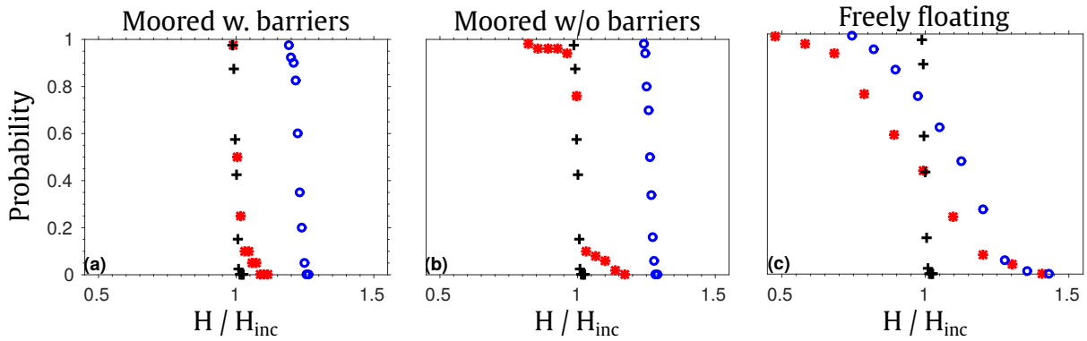
Figure 7: Probability of front-field wave heights exceeding H/H_{inc} , for tests shown in Fig. 6 ( \tau = 0.9 s and ka = 0.12 ). Results for PP plate (*) and PVC plate ( \circ ), with configuration of a (a) moored plate with barriers, (b) moored plate without barriers, and (c) freely floating plate. Results for the incident wave field (+) are included for reference.
