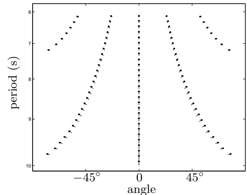
Figure 5. Vectors depicting the components of the energy transmitted by an array composed of one hundred rows. The floes used in the array have mean thickness 1 m and diameter 100 m and the in-row separation is 50 m. The direction of the vectors denotes the angle of the transmitted waves, with the vertical set as being normal to the array, and their magnitudes are derived from the value of the energy carried by the particular wave.
