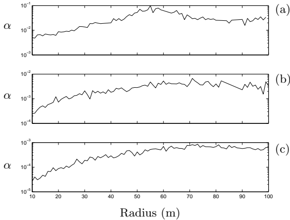
Figure 12. The attenuation coefficient as a function of floe radius for period (a) 8 s, (b) 12 s and (c) 16 s. The floes have mean thickness 1 m and the in-row separation is twenty percent of the radius so that a constant concentration is maintained.
