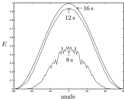
Figure 4. The transmitted energy E as a function of angle after 300 rows. The row geometry is identical to that in figure 3. Wave periods 8 s, 12 s and 16 s are shown (solid lines) along with the energy distribution of the incident wave field (dotted).
