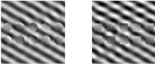
Figure 7. Comparison of the scattering caused by circular floes (left) and square floes (right) when used in two-rows arrays. The figures show ice-floe displacement and water-surface displacement for an obliquely incident ( \chi = \pi/6 ) wave of period 6 s. Although the low wave period distinguishes the relative wave fields, when the number of rows is increased the resulting attenuation coefficients are very similar (0.0378 for an array circles and 0.0535 for an array of squares).
