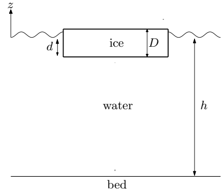
Figure 1. Figure showing the geometry in the vertical plane including a typical floe.
