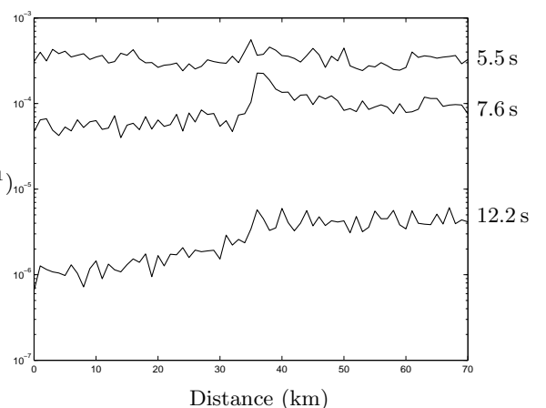
Figure 14. The (dimensional) attenuation coefficient a as a function of distance into the MIZ predicted by our model, where the properties of the ice pack derive from data reported by Squire and Moore [1980].
