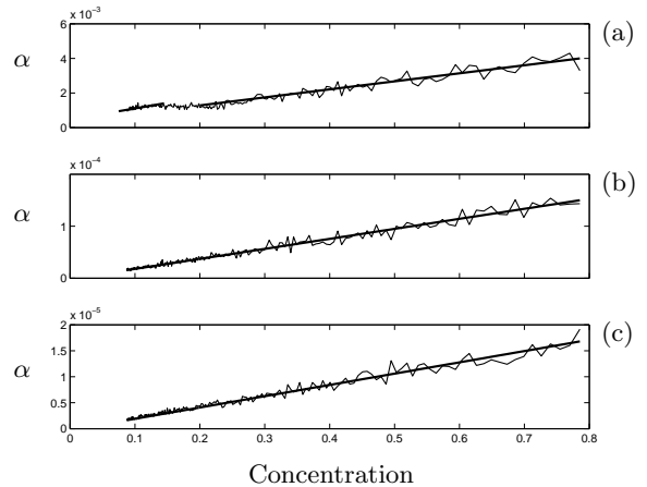
Figure 11. The attenuation shown in figure 10 but as a function of concentration, c , given in equation (4). Straight-line fits are also shown (by thick lines) as described in the text.
