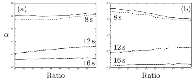
Figure 9. The attenuation coefficient as a function of floe-length ratio when the array is composed of modules containing two floes. Results are shown for three different wave periods and for both square floes (solid lines) and circular floes (broken). Part (a) corresponds to a higher concentration of larger floes while the part (b) is for a lower concentration of smaller floes.
