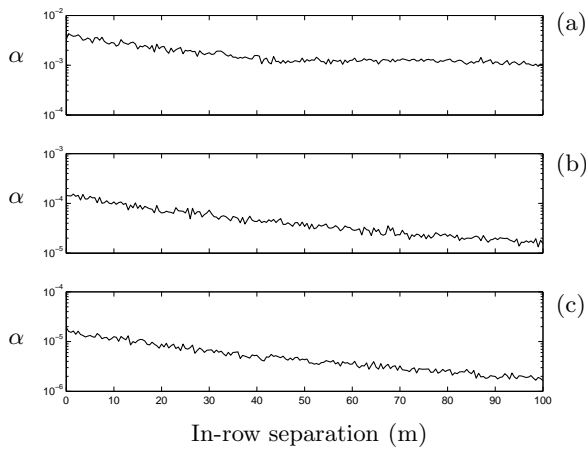
Figure 10. The attenuation coefficient as a function of in-row separation for period (a) 8 s, (b) 12 s and (c) 16 s. The floes have radius 25 m and thickness 0.5 m.
